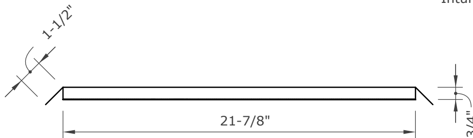
Intumescent Core
