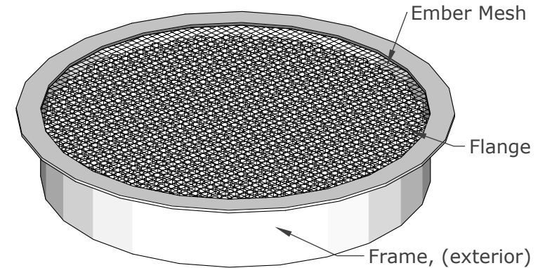
ISOMETRIC VIEW
