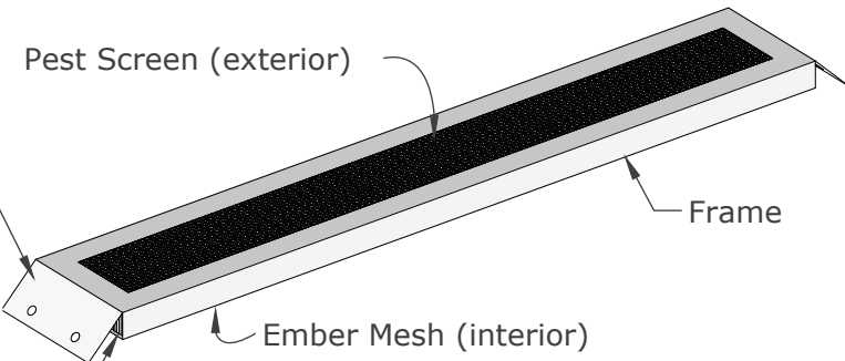
ISOMETRIC VIEW
