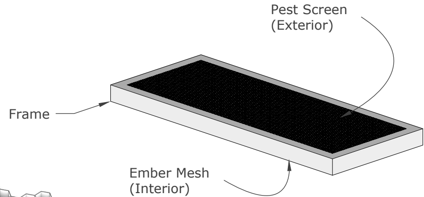
ISOMETRIC VIEW
