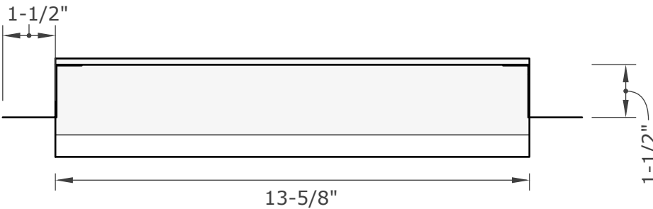
END VIEW
