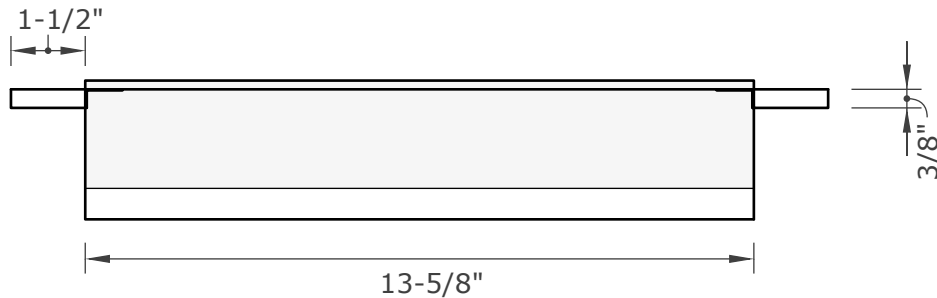
END VIEW
