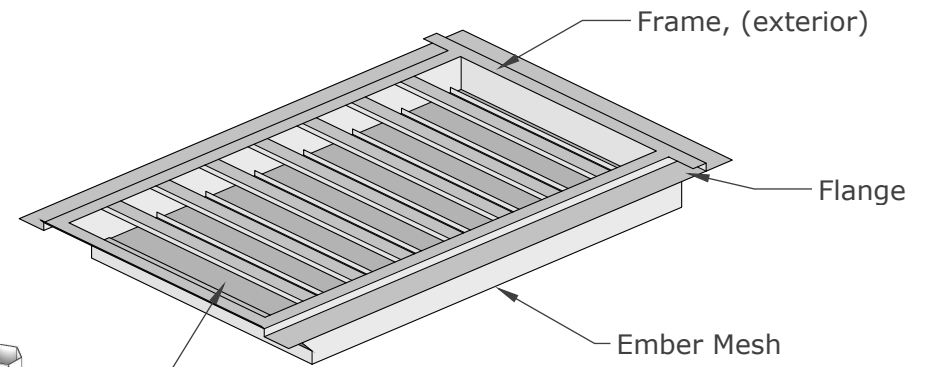
ISOMETRIC VIEW
