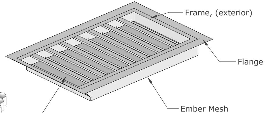
ISOMETRIC VIEW
