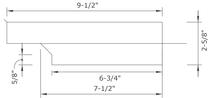
END VIEW
