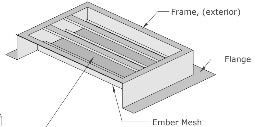
ISOMETRIC VIEW
