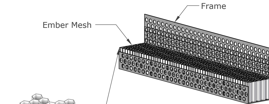
ISOMETRIC VIEW
